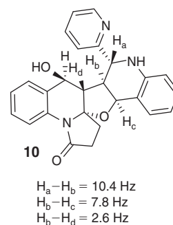
Fig. 3. Spin–spin coupling constants in structures 10 .
