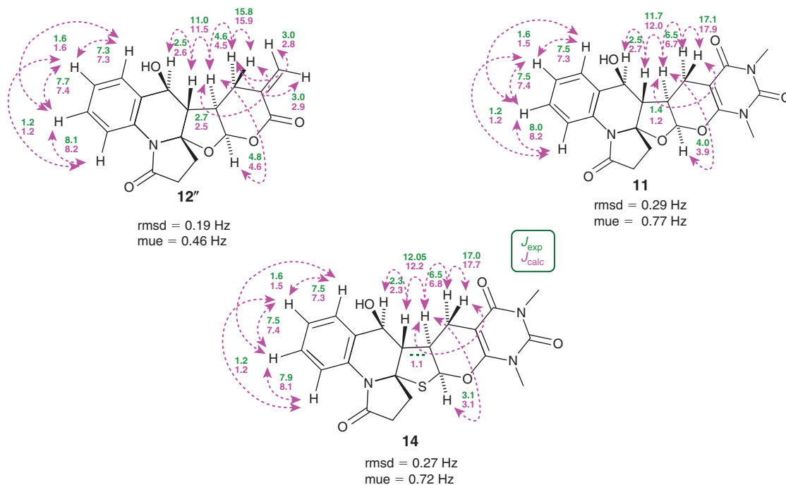
Fig. 4. Comparison of experimental and predicted SSCC for compounds 11, 12'', and 14. rmsd = root-mean-square deviation, mue = maximum unsigned error.
