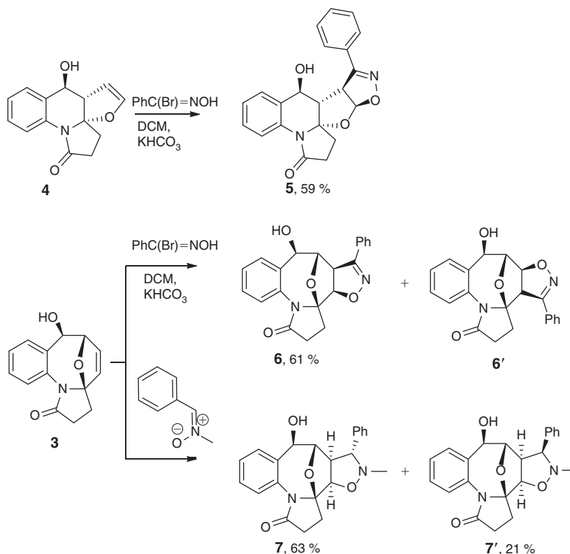
Scheme 3. Reactions with dipoles ( 6' was observed by NMR but not isolated).
