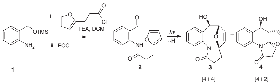
Scheme 2. Synthesis of model compounds. TEA = triethylamine, DCM = dichloromethane, PCC = pyridinium chlorochromate.
