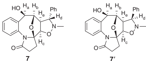
Fig. 2. Nuclear Overhauser Enhancement experiments.
