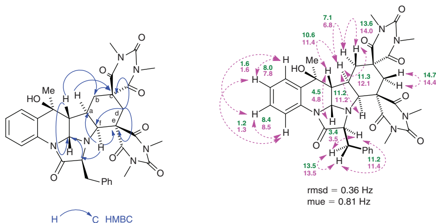
Fig. 5. Selected HMBC relationships between carbon and hydrogen atoms and comparison of calculated and experimental SSCCs for compound 18 .
