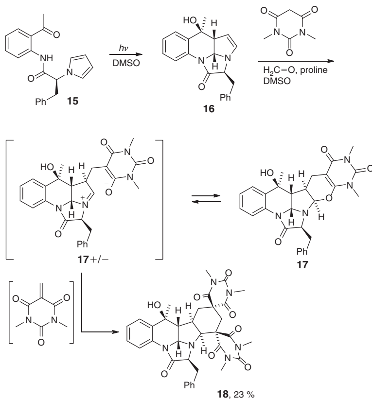
Scheme 7. Reaction with pyrroles.
