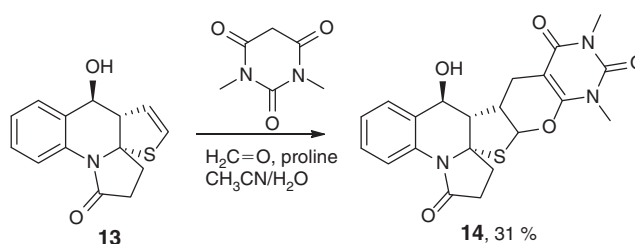
Scheme 6. Thiophene-based [4+2] adduct in the reaction with dimethylbarbituric acid.
