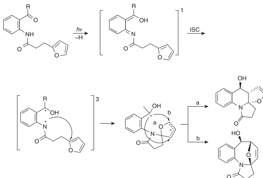
Scheme 1. Photochemical generation of azaxylylenes via ESIP and their intramolecular cycloadditions. ISC = Intersystem crossing.
