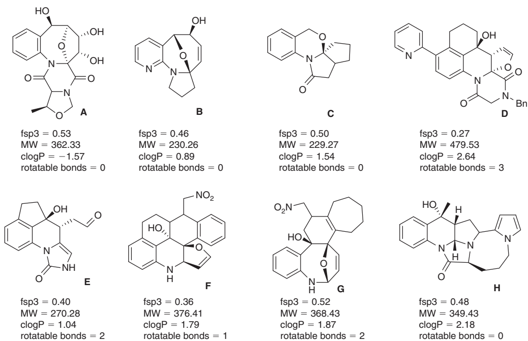
Fig. 1. A subset of diverse molecular scaffolds previously synthesised via intramolecular cycloadditions of photogenerated azaxylylenes.
