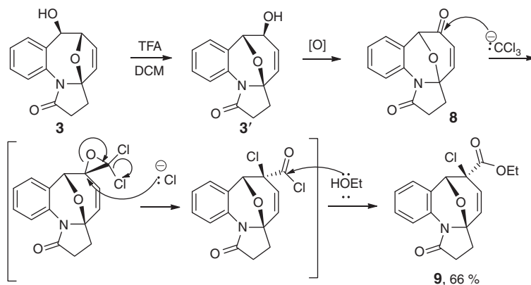
Scheme 4. Addition of dichlorocarbene to \alpha,\beta -unsaturated ketone 8 . TFA = trifluoroacetic acid.
