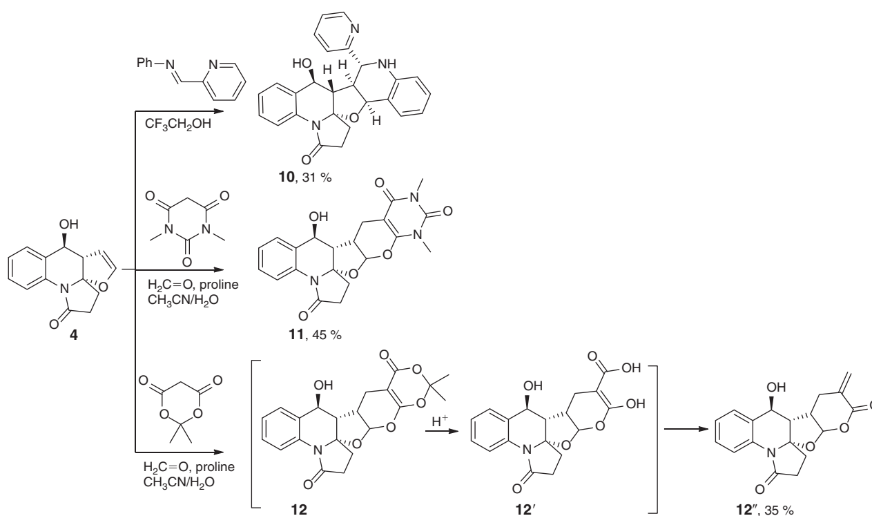
Scheme 5. Postphotochemical [4+2] cycloadditions of heterodienes to primary photoproducts.
